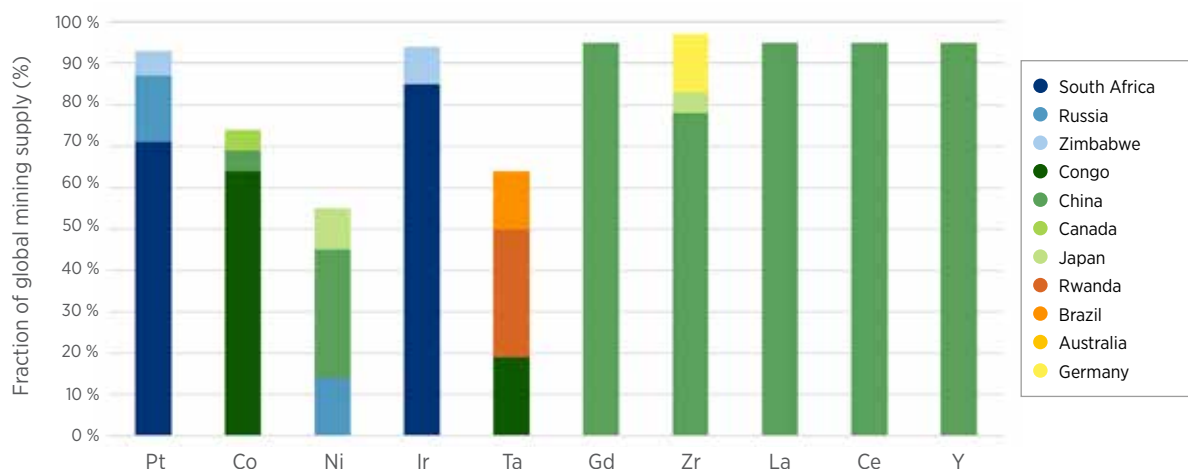
Figure 24. Top producers of critical materials in electrolysis.
