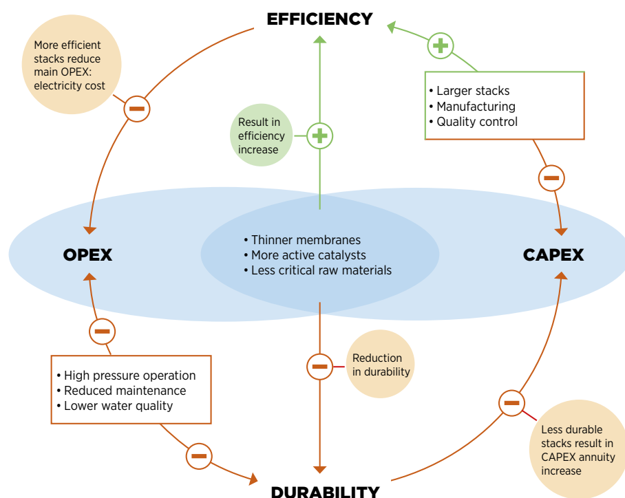
Figure 14. Trade-offs between efficiency, durability and cost for electrolysers.
