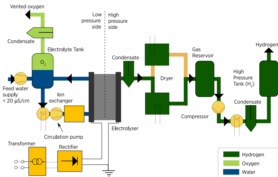
Figure 9. Typical system design and balance of plant for an AEM electrolyzer.
