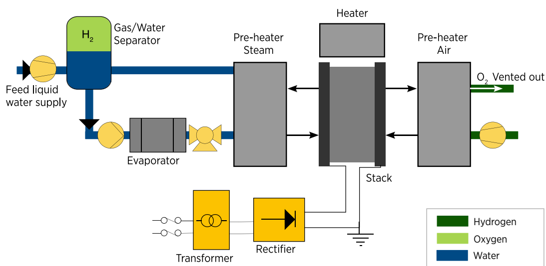
Figure 10. Typical system design and balance of plant for a solid oxide electrolyzer.
